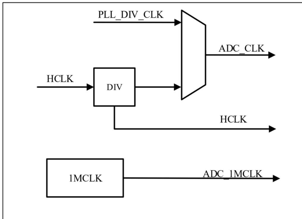
Figure 2-1 ADC Clock
