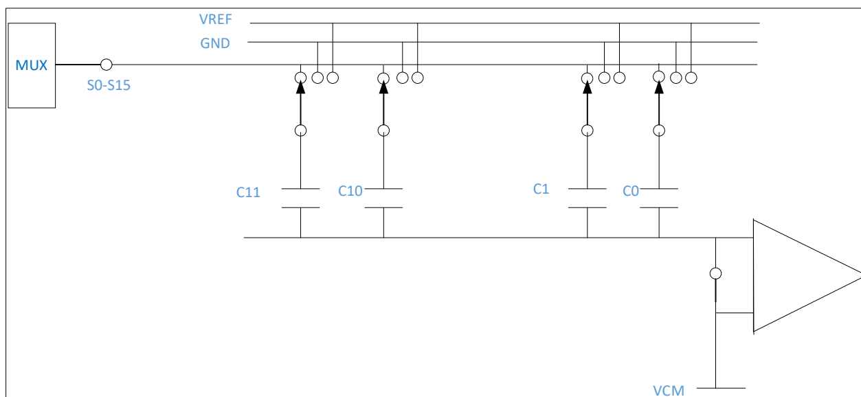
Figure 1-2 Equivalent Circuit of Sampling Stage
