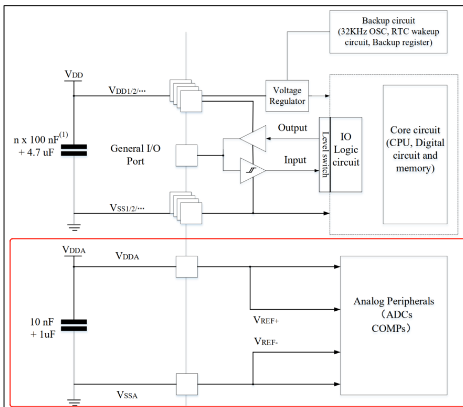
Figure 2-6 Power System
